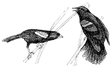
Figure 3. Red-winged Blackbirds.
